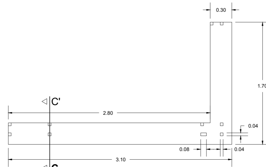
Balcão 2
