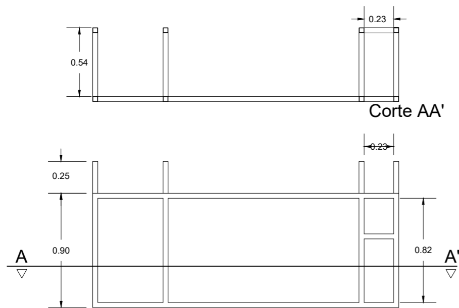
Vista Principal
